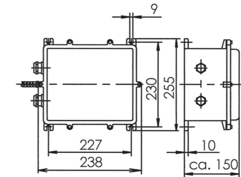
VKA 400/50/So/IP68/k
